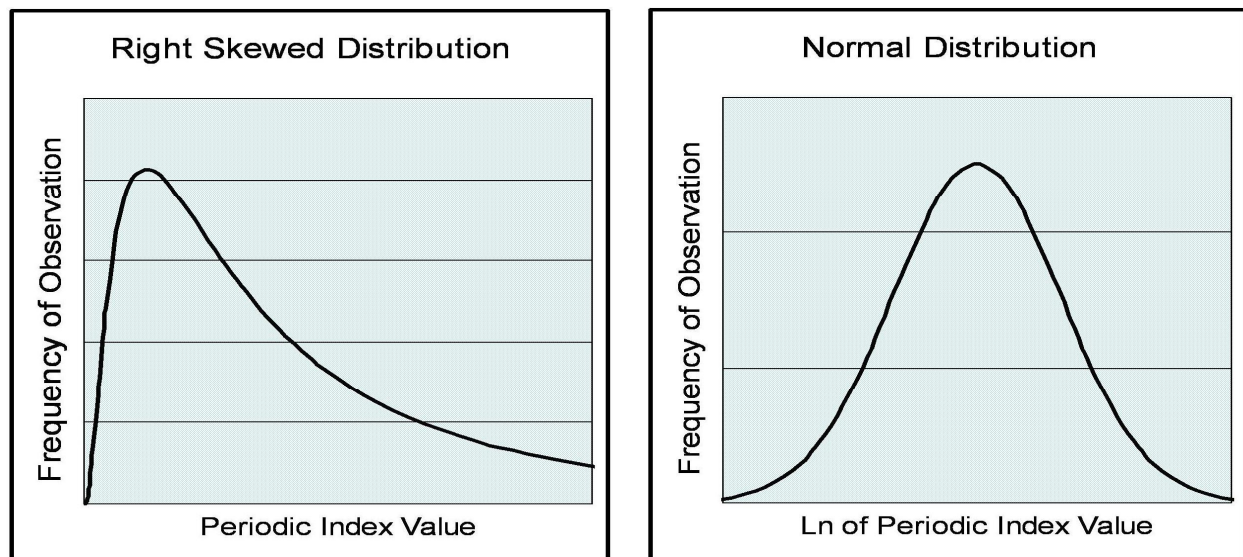
Figure 1. Right-Skewed & Normal Distributions
