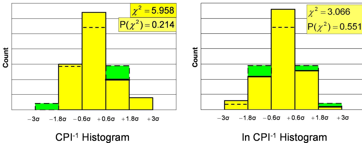
Figure 2. Histograms
